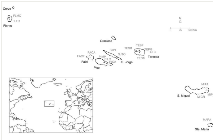
Figure 1. Location of the Azores and of native forest fragments in the archipelago. Codes for forest fragments as in Table 1.
