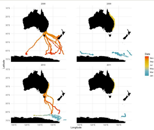
Figure 3. State-space model location estimates generated by satellite tagged east Australian (breeding stock E1) humpback whales in each year and coloured according to month.
