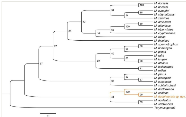
Figure 4. Phylogenetic trees of Megastigmus inferred by Maximum Likelihood (ML) methods, based on mitochondrial data ( COI + Cytb ).
