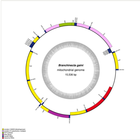
Figure 1. Circular map of the mitochondrial genome of Branchinecta gaini . Genes drawn inside the circle are transcribed in a clockwise and genes drawn outside the circle are transcribed in a counterclockwise direction. The inner grey circle shows the GC content.
