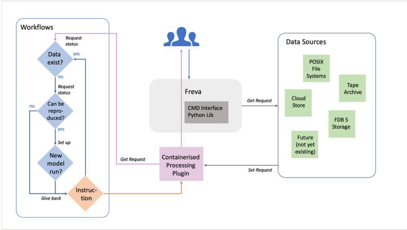
Figure 1. Next development steps within Freva.
