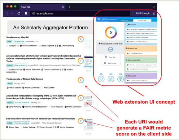
Figure 1. The FAIR extension mock UI concept.
