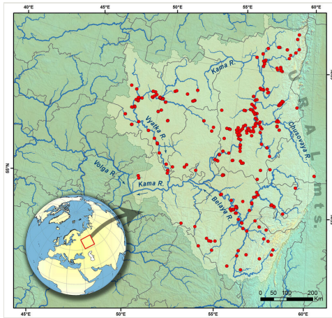
Figure 1. Map of sampling sites in the Kama River Basin. The map was created in ArcGIS 10.8 software ( www.esri.com ).
