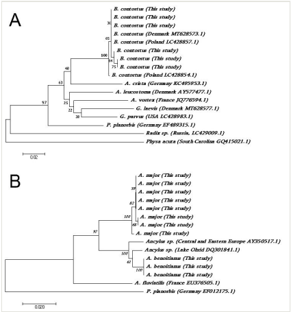
Figure 4. Neighbour Joining trees. A. Bathymophalus contortus (16S rRNA mt gene fragment); B. Ancylus spp. (COI mt gene fragment). GenBank Accession numbers and sample origin places are indicated for downloaded sequences. Branch length (and scale-bar) resembles the nucleotide divergence (K2P distance) and the numbers at the node indicates bootstrap support after 100 permutations.
