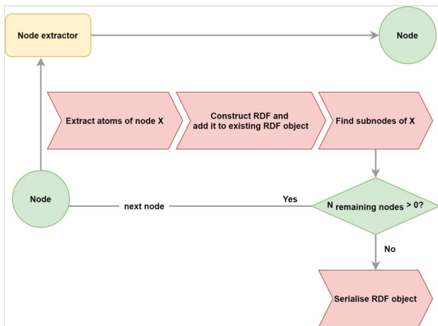
Figure 3. The Extractor procedure
