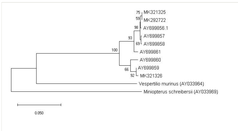
Figure 8. Maximum Likelihood tree (Tamura-Nei model).
