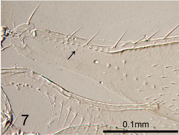
Figure 7. Cales motterni : detail of basal fore wing showing campaniform sensilla (arrowed)
