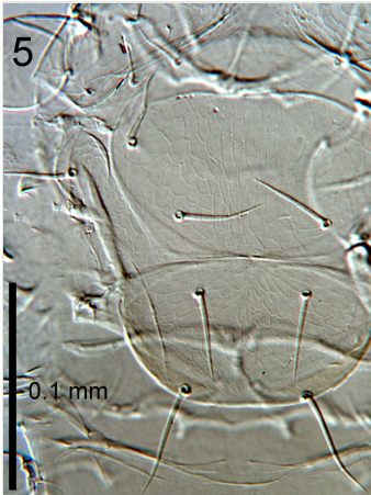
Figure 5. Cales motterni : mesoscutum and scutellum
