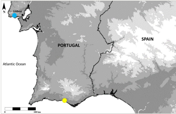
Figure 3. Distribution map of the Miomantis spp. citations in this work. Miomantis paykullii - yellow circle. Miomantis caffra - blue circle.
