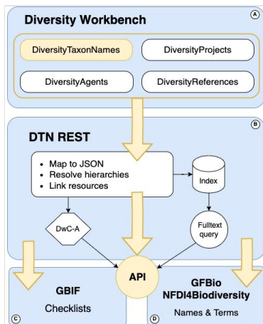
Figure 1. Generic data management and publication in four steps (A-D) as applied for the IPM taxon reference list (Novotný et al. 2022)
