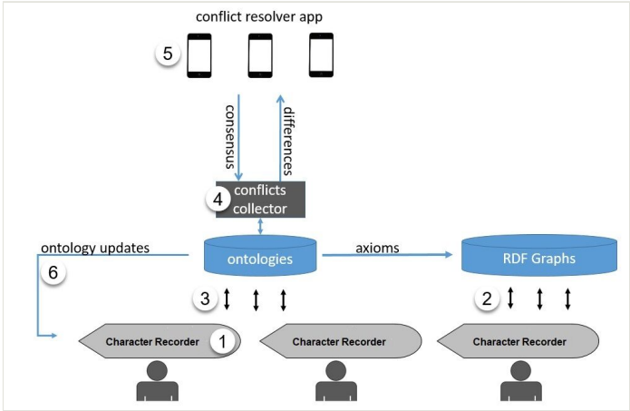
Figure 1. System diagram for the author-driven computable data and ontology development platform.
