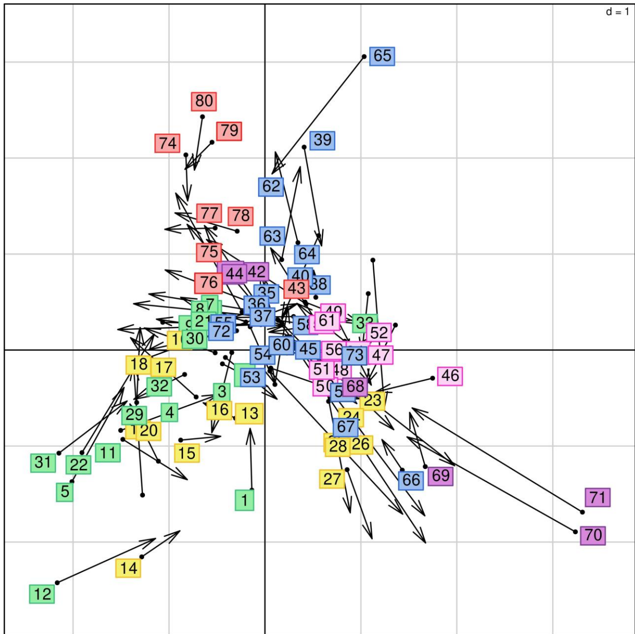
Co-inertia: position of the plots sampled. The beginning of the arrow is the position of the plot described by the environmental data set; the end of the arrow is the position of the site described by the fern abundance.
