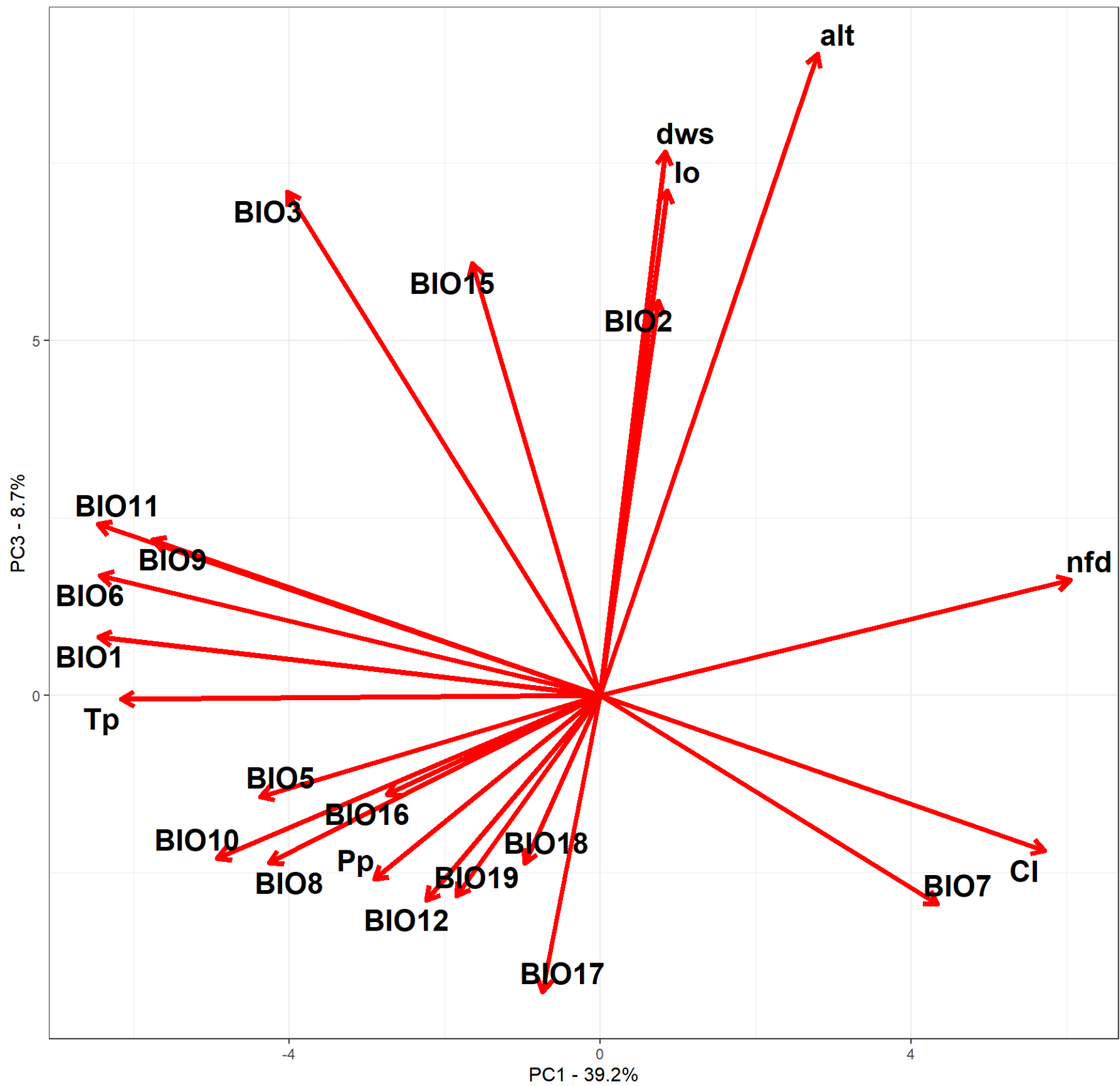
Variable vectors PC1 - PC3
