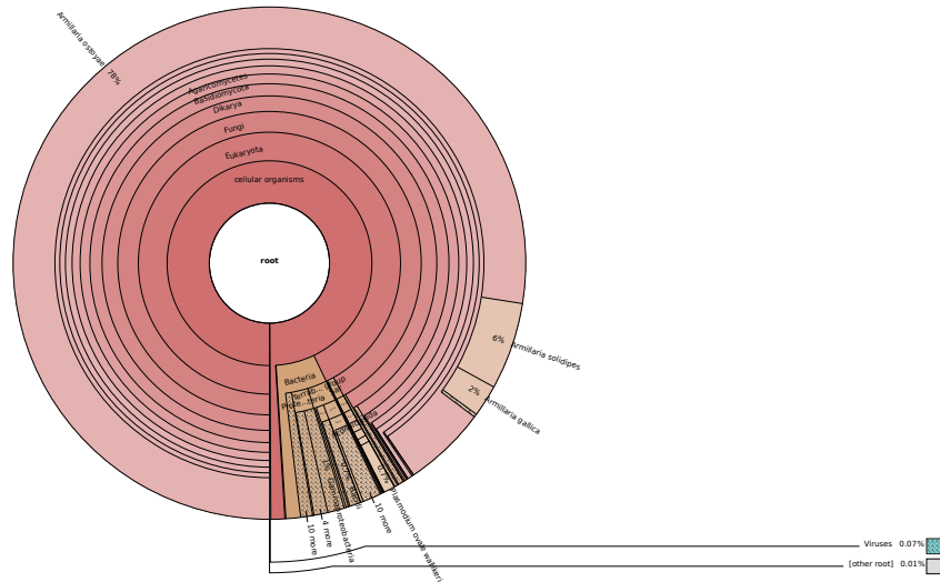
S1b : Proportion of the Armillaria genome assembly assigned to different taxa using Kaiju
