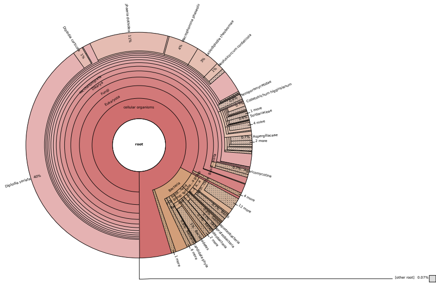
S1a : Proportion of the Diplodia genome assembly assigned to different taxa using Kaiju
