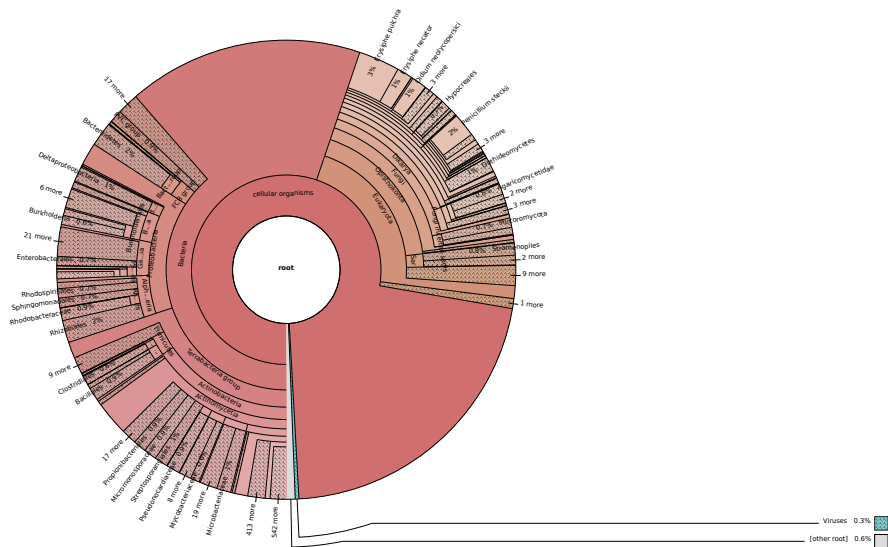
S1c : Proportion of the Erysiphe genome assembly assigned to different taxa using Kaiju
