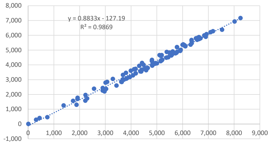
Correlation of fungal loci and loci in final dataset
