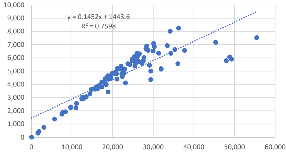
Correlation of loci before and after mapping
