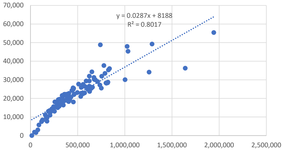
Correlation of reads and clustered loci
