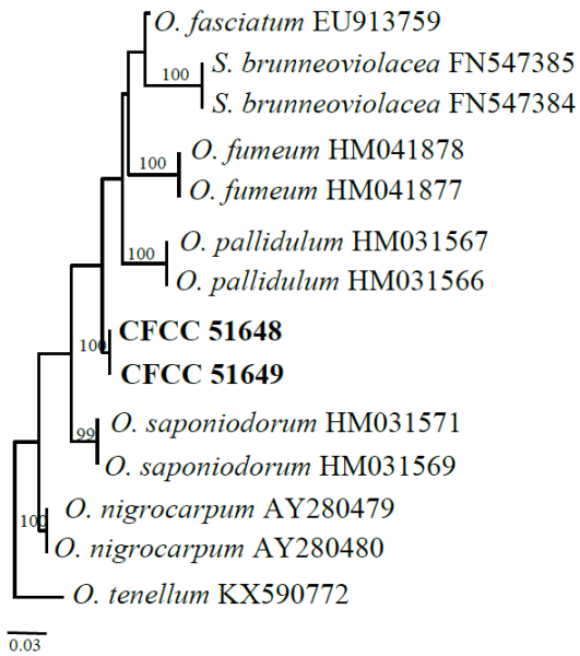
Appendix Fig 3: Three ML phylogenetic trees based on tub2 after excluding introns.
