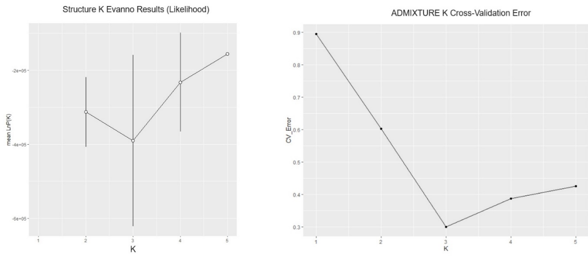
Figure S1. SNPs cluster evaluations in STRUCTURE and ADMIXTURE.
